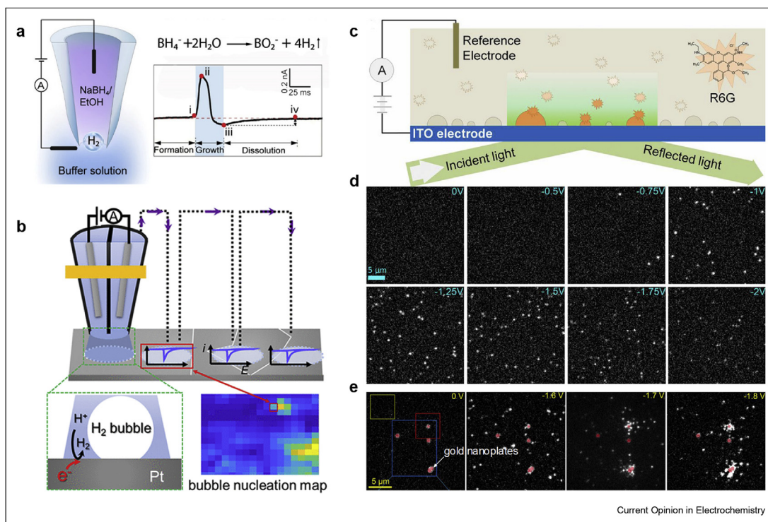
a) Schematic of the experimental setup for analyzing the dynamics of chemically generated nanobubbles using a nanopore, and a typical current–time trace showing the formation (i), growth (i–iii), and dissolution (iii–iv) of a nanobubble. (b) The SECCM setup for mapping the H 2 bubble nucleation conditions on an electrocatalytic surface. A nanopipette/droplet probe is drawn near and retracted at different locations to obtain local voltammograms of bubble nucleation. (c) Schematic of the experimental setup utilized for imaging surface H 2 nanobubbles during electrocatalytic water splitting. H 2 nanobubbles generated on an indium tin oxide (ITO) surface are labeled by single rhodamine 6G molecules and imaged by total internal reflection fluorescence microscopy. (d) A series of fluorescence images of an ITO electrode taken during a potential scan from 0 V to –2.0 V vs. Pt quasi-reference electrode. (e) Fluorescence images showing H 2 nanobubbles on a gold nanoplate–decorated ITO electrode in the water at a potential from +0.5 V to –1.8 V vs. Pt quasi-reference electrode. Adapted with permission from a study by Hu et al. [27] and Wang et al. [32] copyright (2018 and 2019) by the American Chemical Society, and from a study by Hao et al. [43], copyright (2018) by the National Academy of Sciences.
